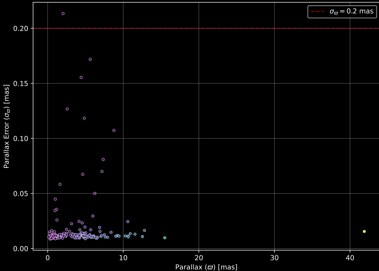
APOGEE DR17 Field: [CVZTILE_091+24_btx] Parallax Quality (n= 170)
