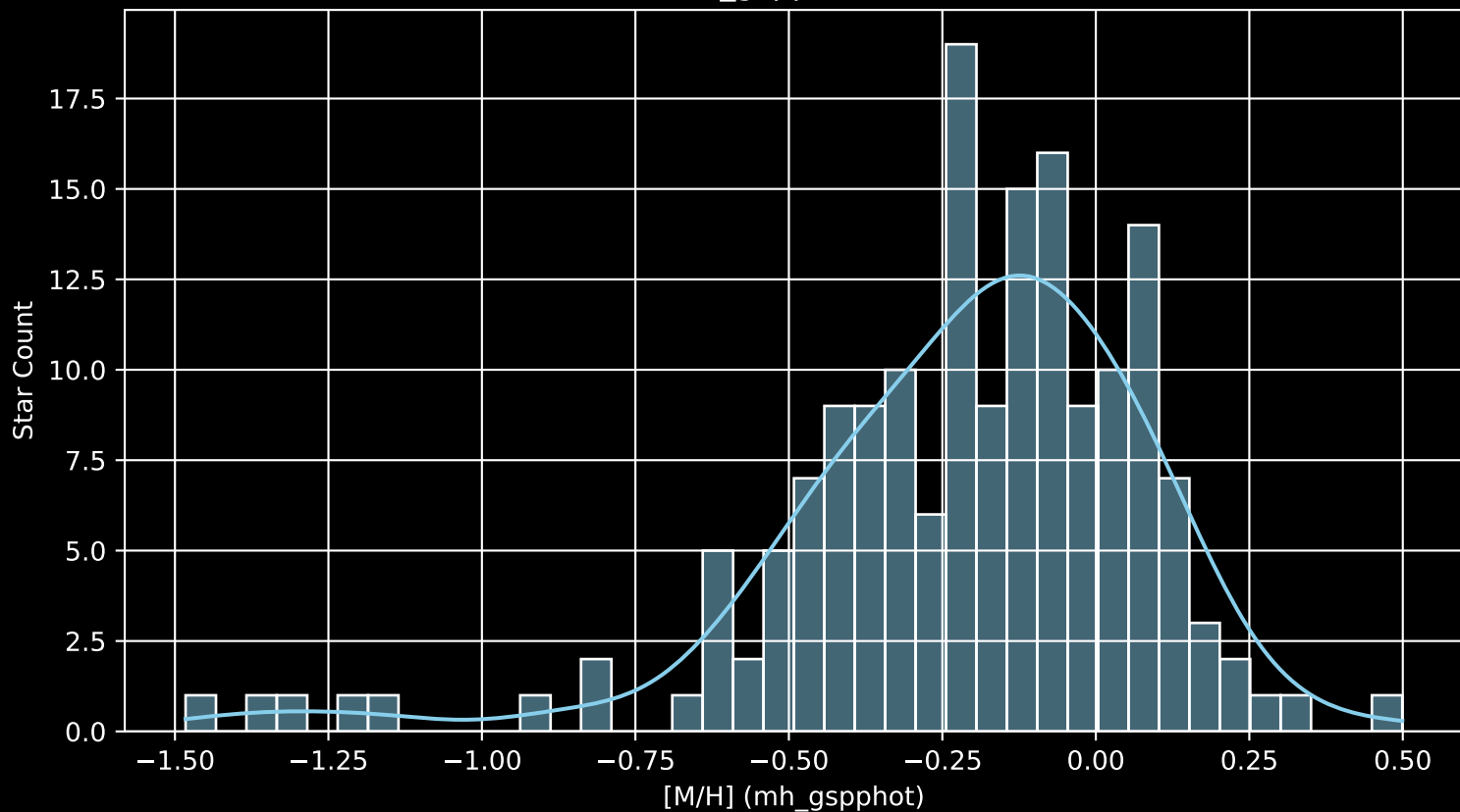
APOGEE DR17 Field: [CVZTILE_091+24_btx [M/H] (mh_gspphot) (n= 169)
