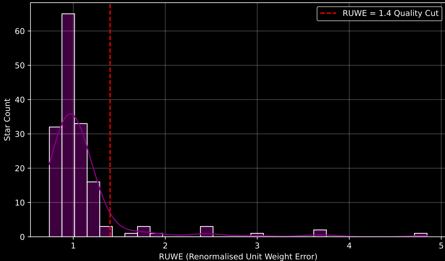
GAPOGEE DR17 Field [CVZTILE_091+24_btx] RUWE Distribution (n= 161)
