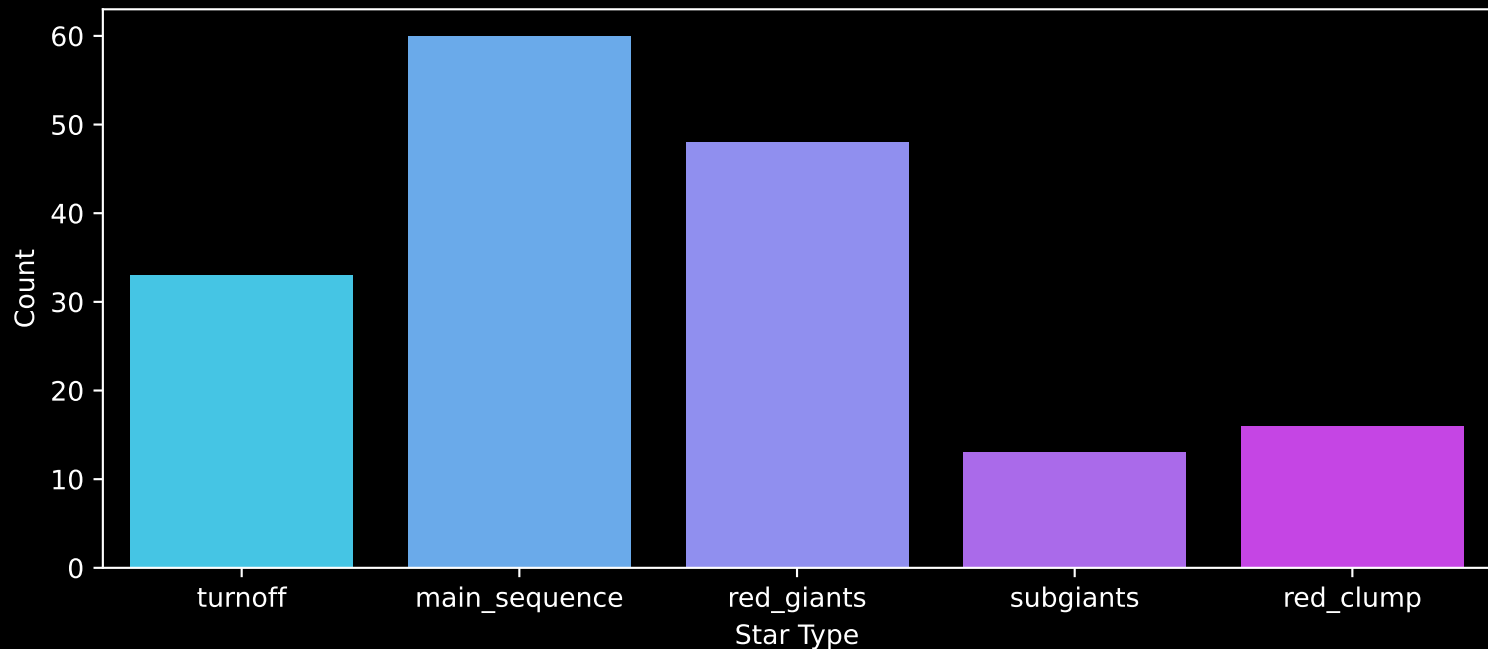
APOGEE DR17 Field: [CVZTILE_091+24_btx] Count plot of Star Type
