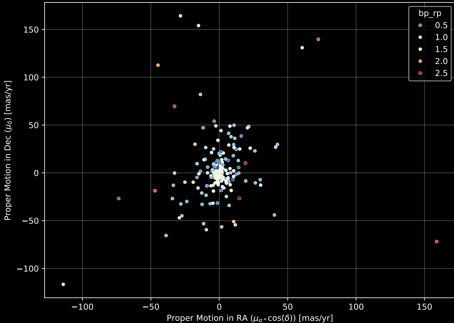
APOGEE DR17 Field: [CVZTILE_091+24_btx] Proper Motion Diagram (n= 170)
